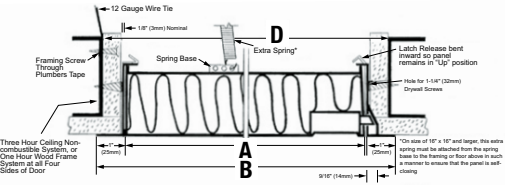
3-hour Ceiling Installation Models FD and FDSS
