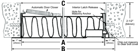
Wall Installation Models FD, FDSS, and HGFD
