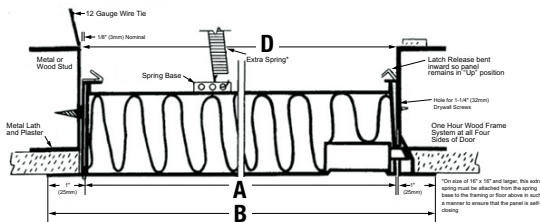
1-hour Ceiling Installation Models FD and FDSS
